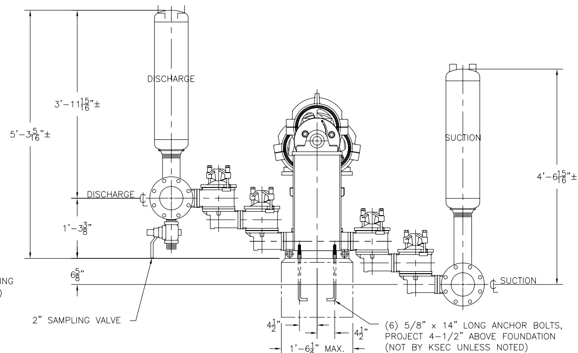
FRONT ELEVATION LEFT HAND PUMP
