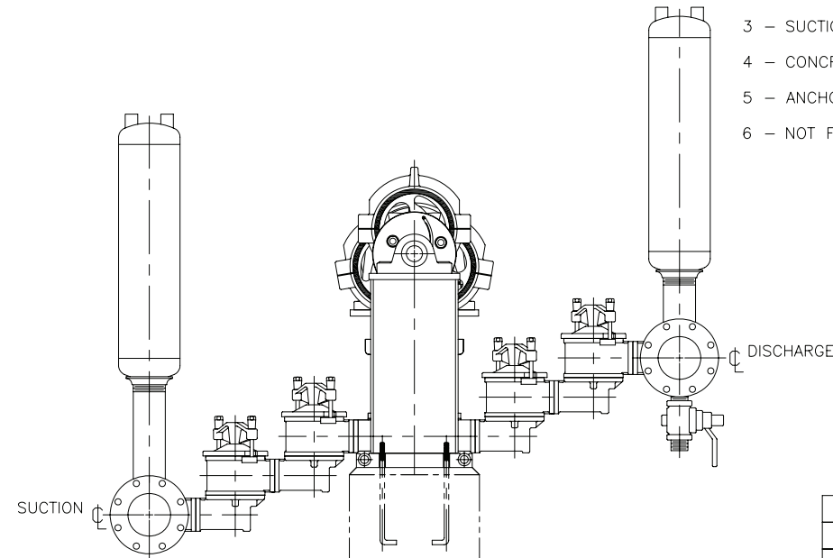
FRONT ELEVATION LEFT HAND PUMP
